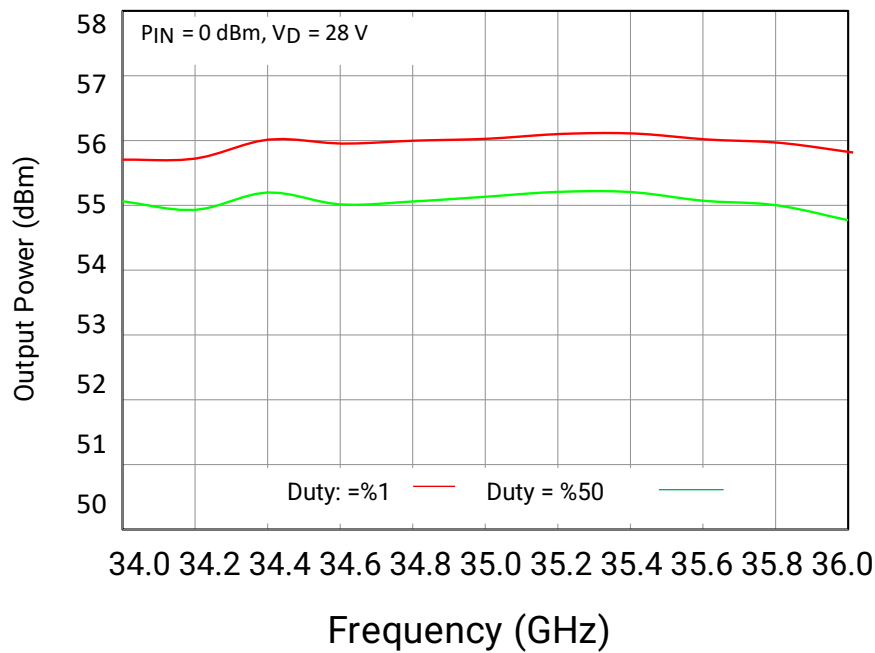
Output Power vs. Freq.
